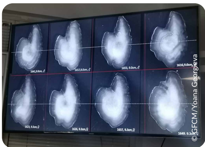
Experts presenting European sprat age reading.
